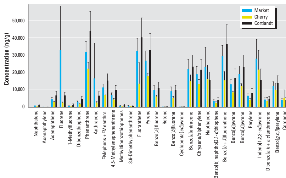
Figure 7. PAH concentrations measured in the Cortlandt, Market, and Cherry Street samples [average PAH concentrations \pm 1 SD ( n = 3 )]. 2 Mephens + 2 Meanthrs, \Sigma methylphenanthrenes + \Sigma methylanthracenes.
